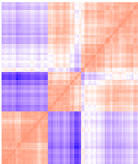
Clustering tendency
