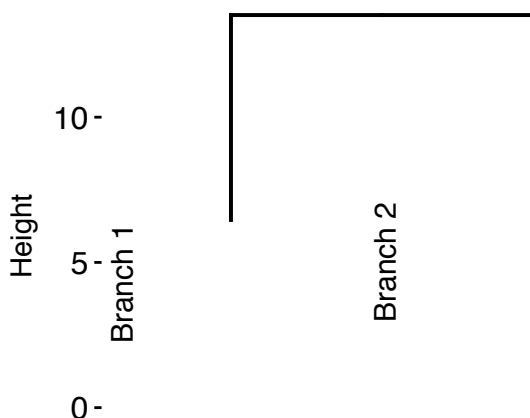
Cluster Dendrogram
