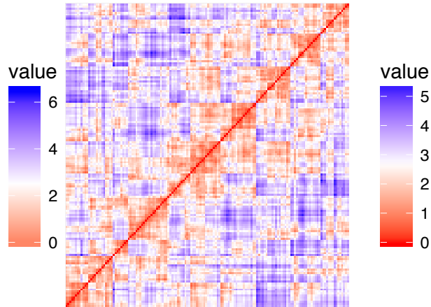
Random data
